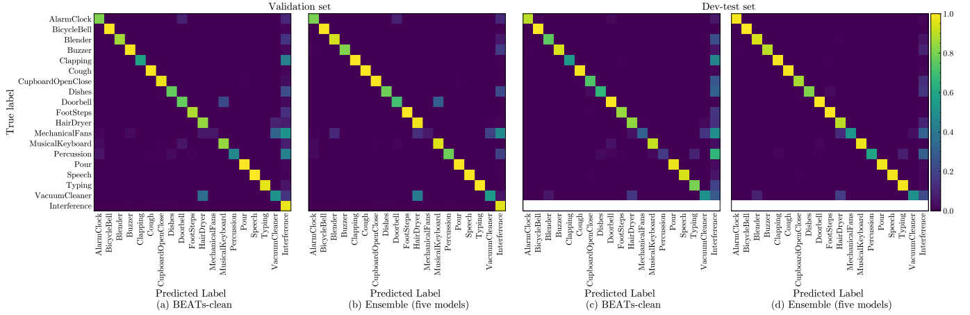
Fig. 2: Confusion matrices for BEATs-clean (the first row in Table 3) and ensemble of the five models (the last row in Table 3) with row-wise normalization. For this figure, no sources were discarded even when four or more sources were estimated as target sources.
