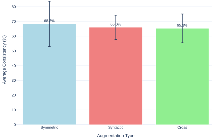
Figure 35: Average consistency rates by augmentation strategy across 41 vision-language models with 4-variant question sets. Error bars represent standard deviation across models. Symmetric augmentations (question reformulations maintaining logical equivalence) achieve slightly higher consistency than syntactic (surface-level rephrasing) and cross-augmentation (mixed transformations) approaches.
