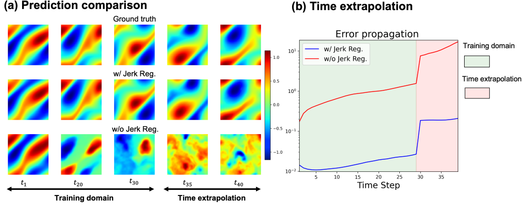
Figure 4: Comparison of ground truth vorticity fields and model predictions. (a) Time interpolation and extrapolation comparisons in the test set. (b) Relative mean square error (RMSE) inside (green area) and outside (pink area) the training time domain.
