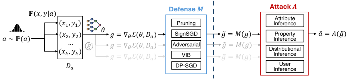
Figure 1: Overview of the unified inference game from gradients: the adversary infers the sensitive variable a from observations of the gradients \tilde{g} computed on the private data batch \mathcal{D}_a .
