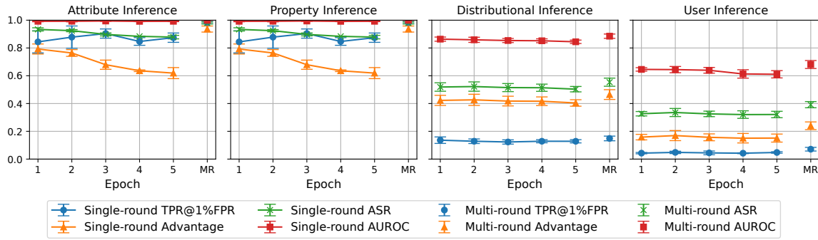
Figure 2: Comparison of single-round and multi-round inference attacks on the Adult (AIA, PIA, DIA) and CREMA-D (UIA) datasets. A complete result on all datasets is provided in Appendix B.2.
