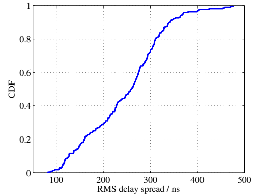
Fig. 5. CDF of RMS delay spread with threshold of 60 dB below maximum
